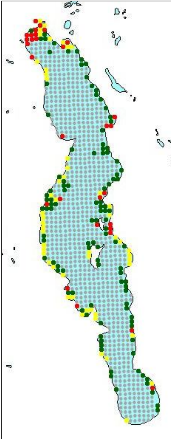
Rake Density-Green = 1, Yellow =2, and Red = 3.
